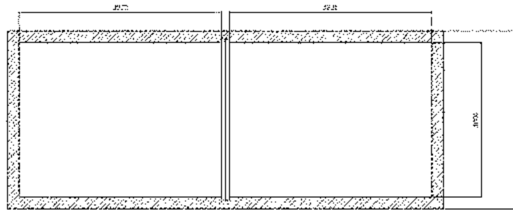
SECTION 8-E SCALE 1:10
